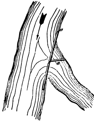
Fig. 252.—A lateral floating boom.
